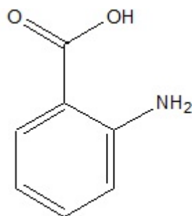
Anthranilic Acid
