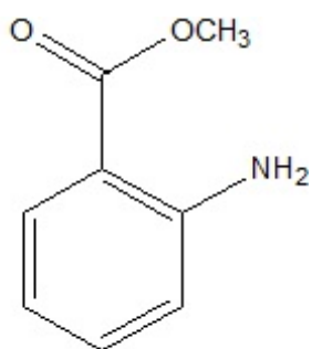
Methyl Anthranilate
