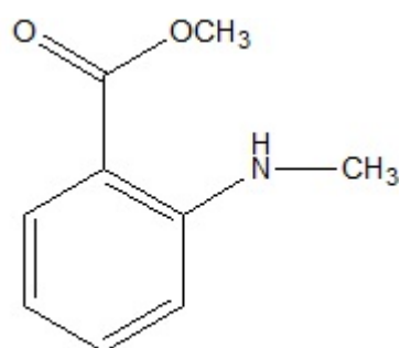
Dimethyl anthranilate
