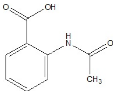
N-Acetylanthranilic acid
