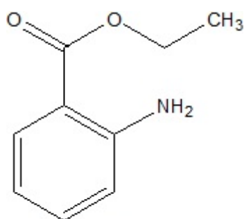
Ethyl Anthranilate
